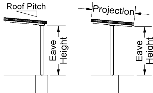
Full Cantilever
